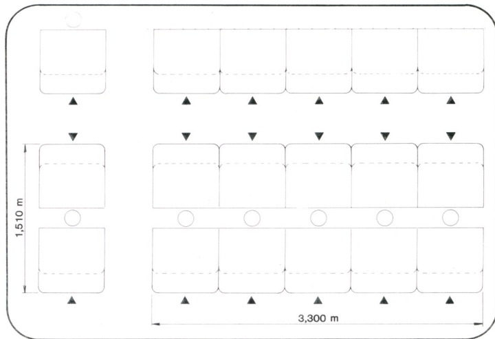
implantation
